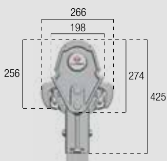
Dimensions with Texpro profile
