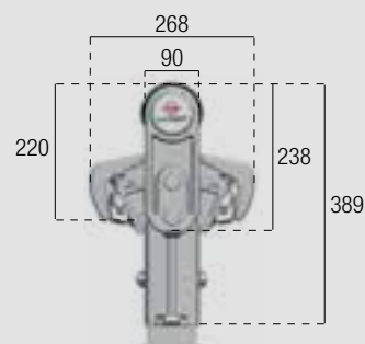
Dimensions without Texpro profile
